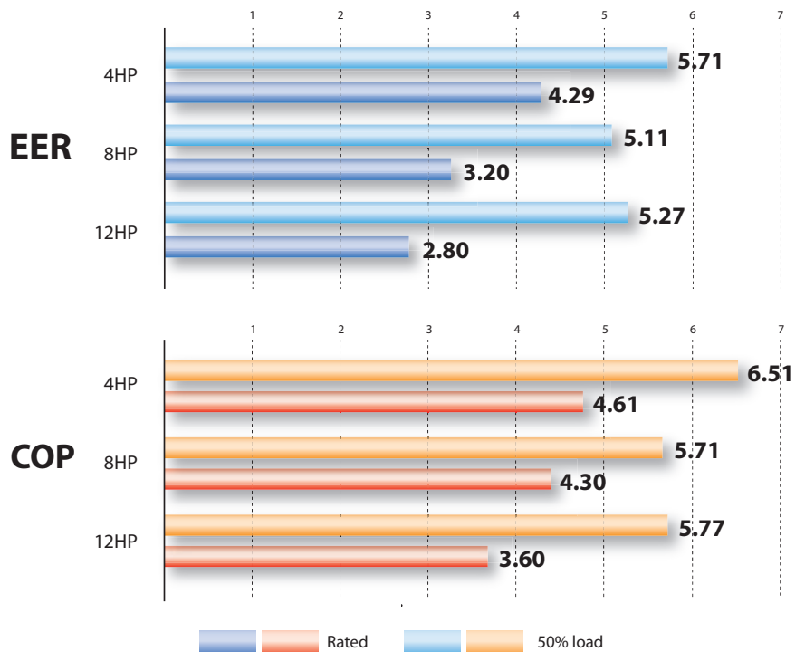
4HP: MCY-MAP0401HT/HT2D 8H P: MCY-MAP0804HT8/HT7 12H P: MCY-MHP1204HT8
