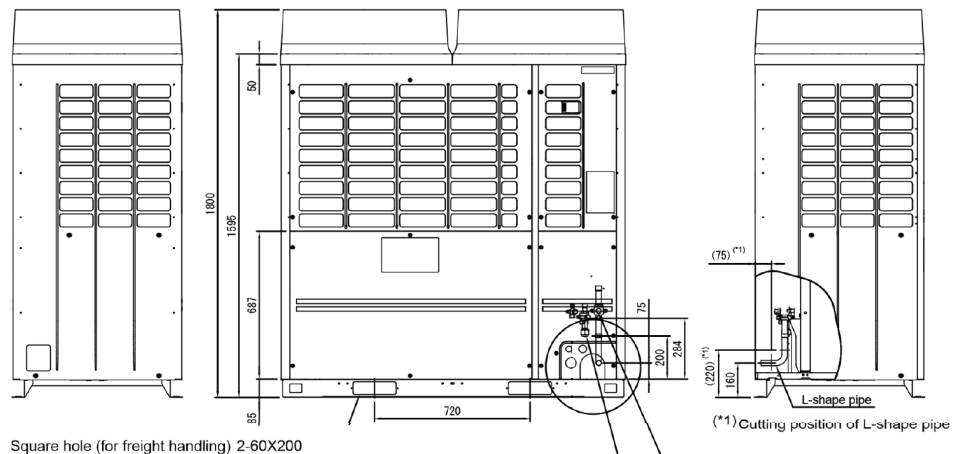
Gas pipe connection port \phi_A
